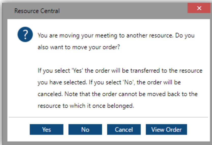
Figure 12. Message dialog
