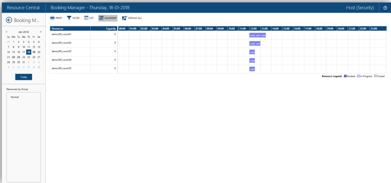
Figure 2. Booking Manager
