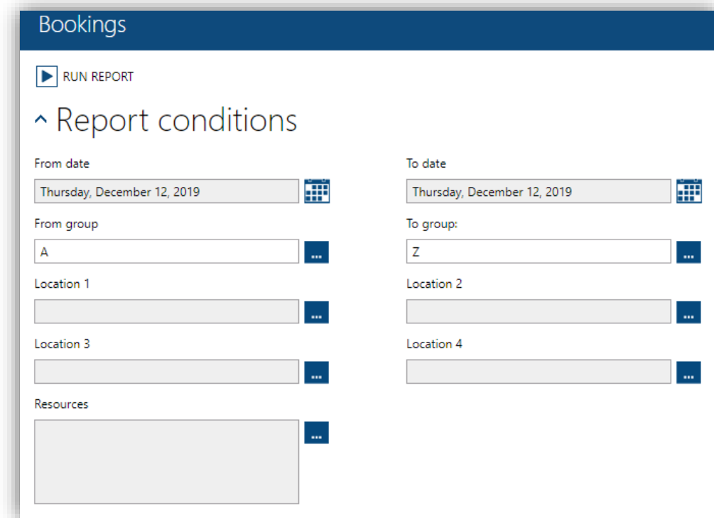
Figure 196. Bookings report
