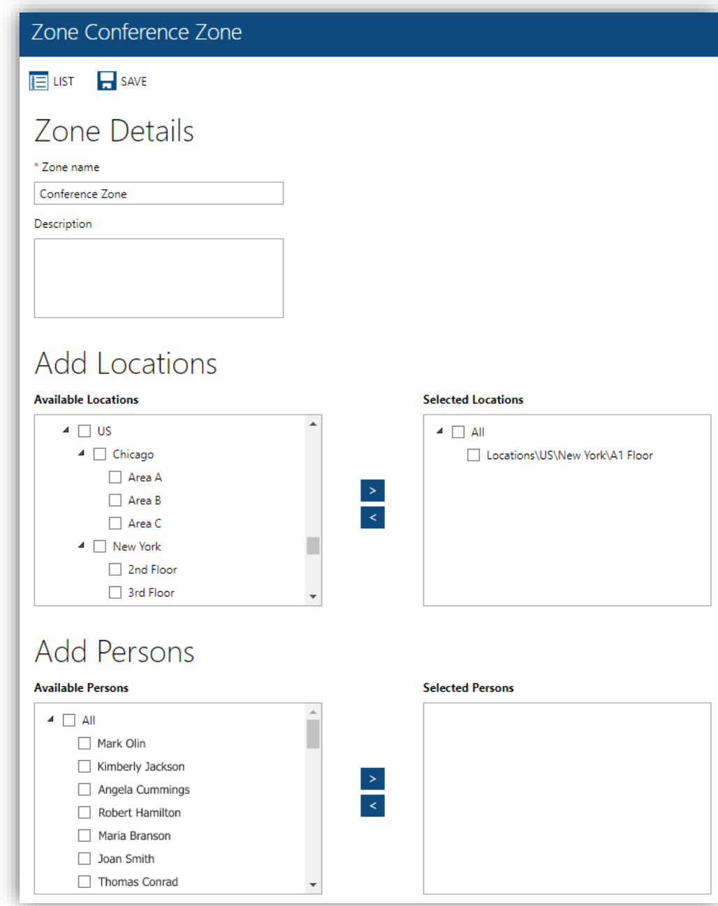
Figure 336. Zone details
