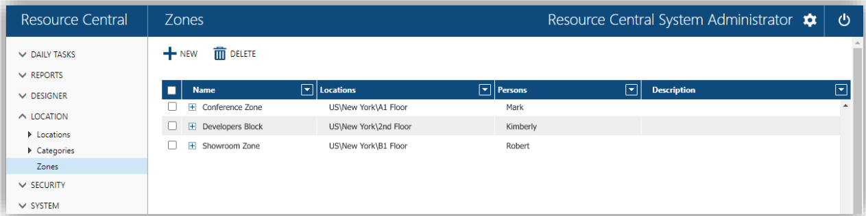
Figure 335. Zones list
