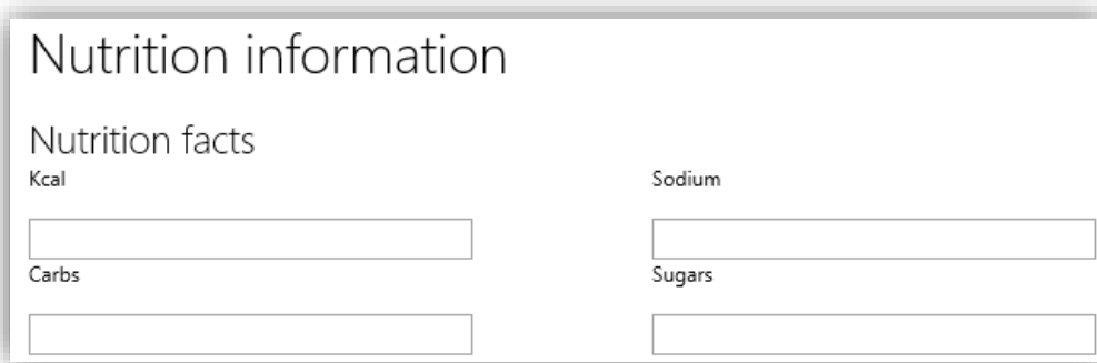
Figure 271. Datatype – Numeric
