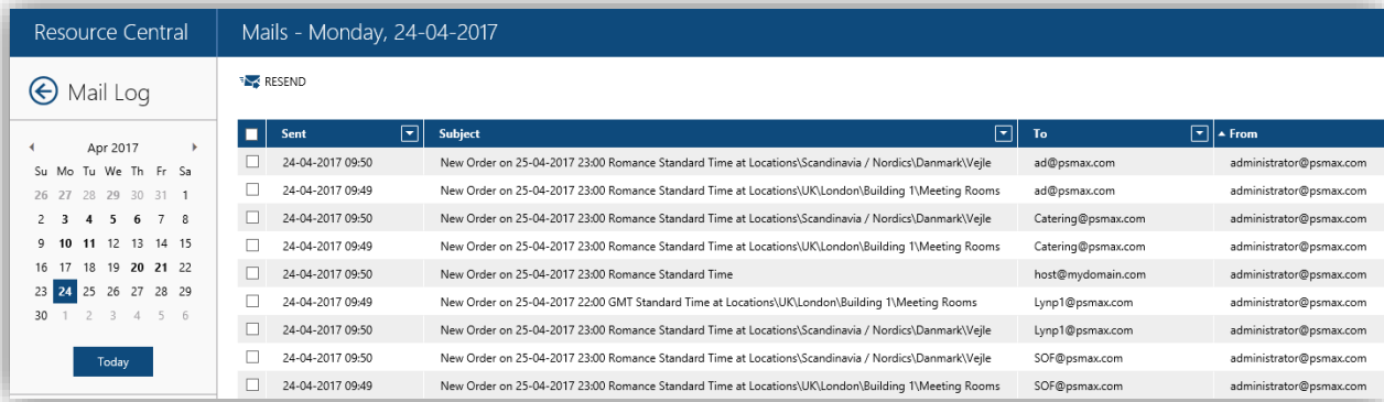
Figure 371. Mail Log
