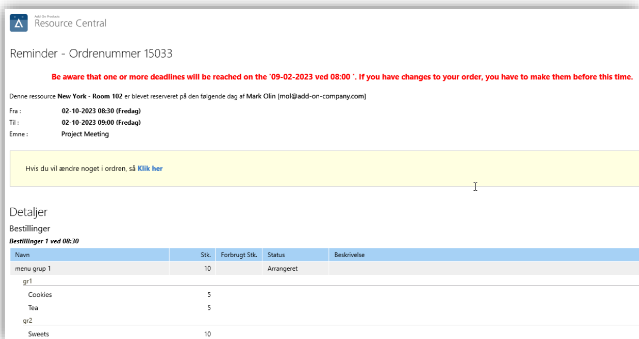
Figure 161. Reminder email
