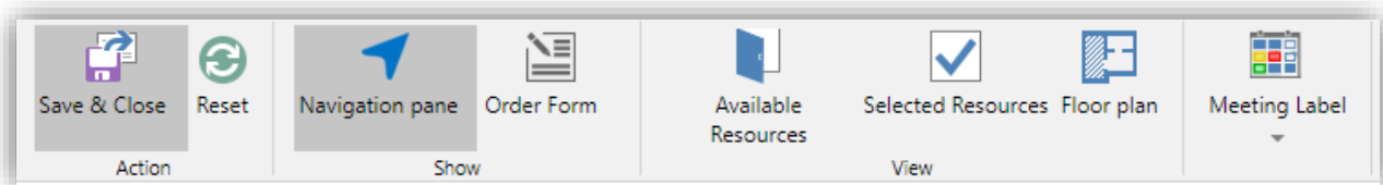
Figure 5. ResourceFinder Toolbar
