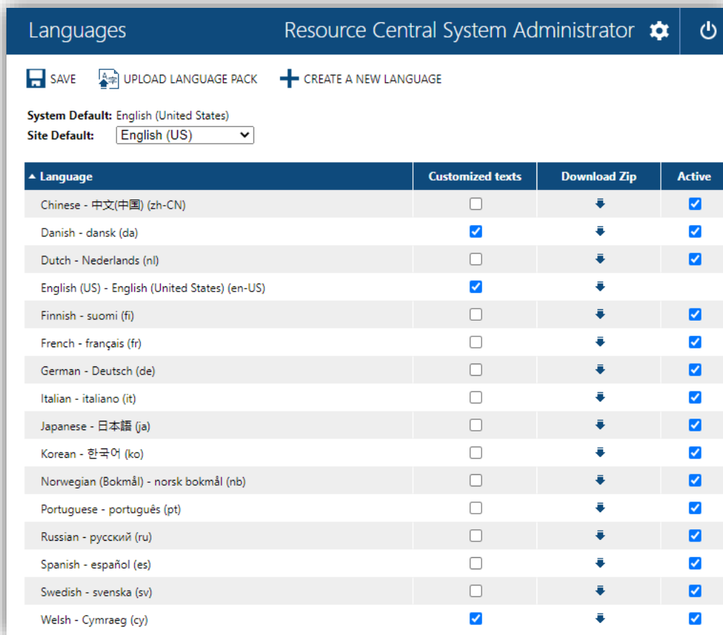
Figure 360. Languages section
