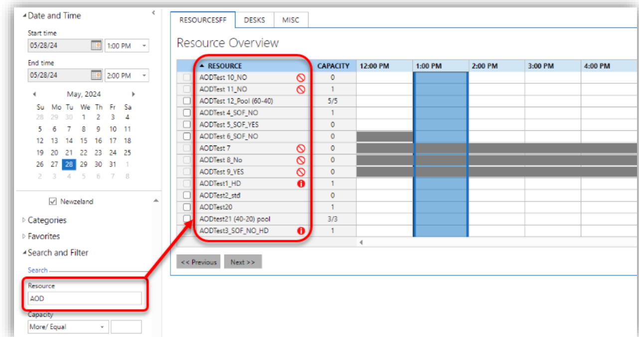
Figure 37. Search
