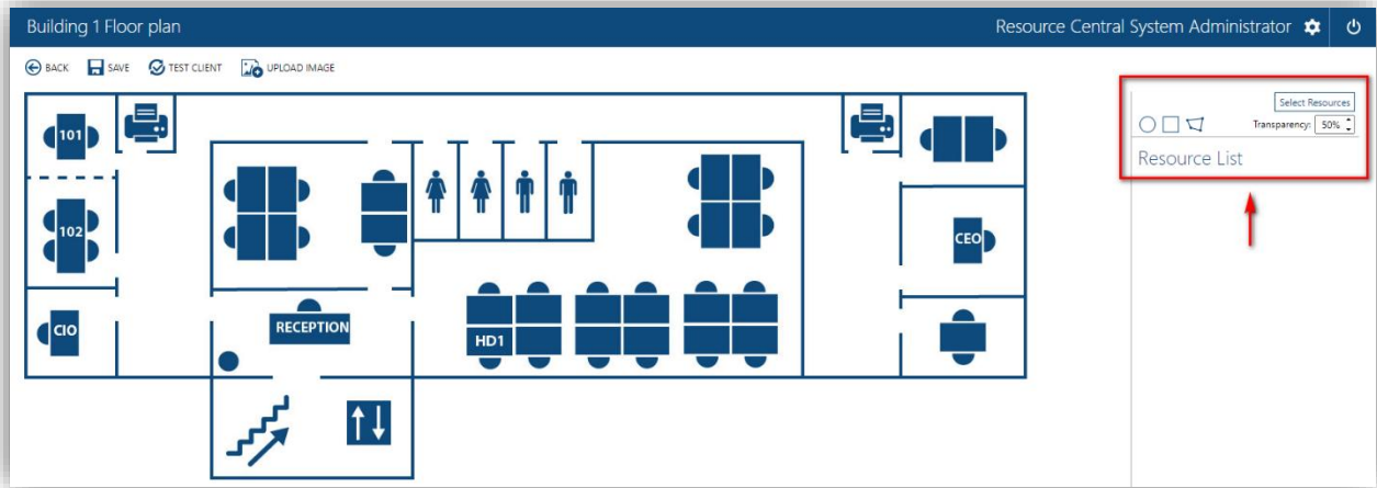
Figure 316. Resource mapping
