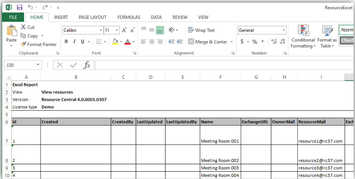
Figure 223. Resources Excel
