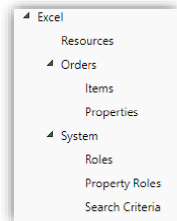
Figure 221. Excel
