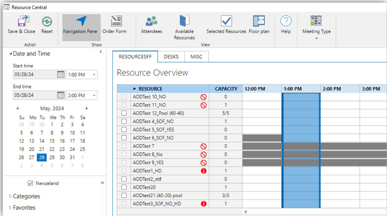
Figure 25. ResourceFinder window
