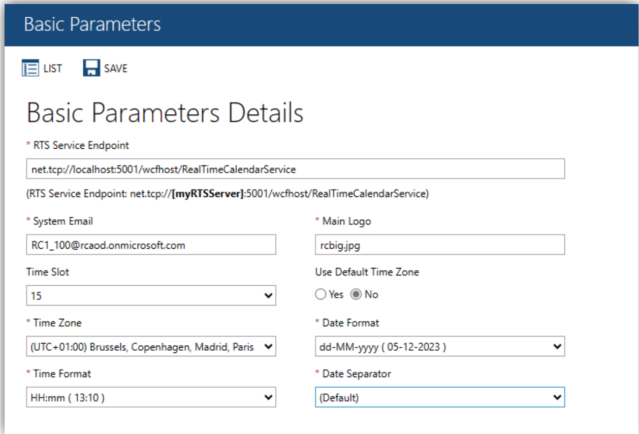
Figure 356. Basic parameters
