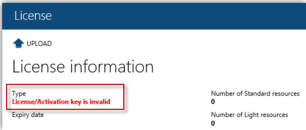
Figure 379. License
