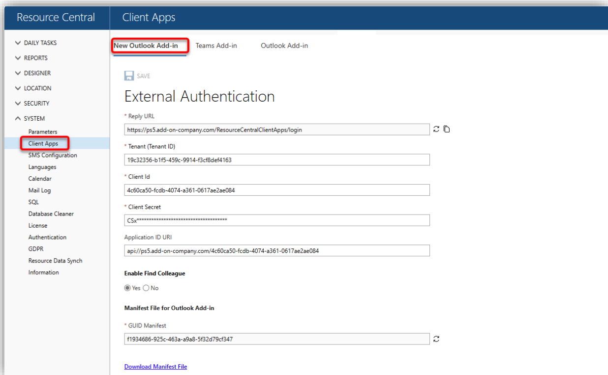
Figure 358. Client Apps
