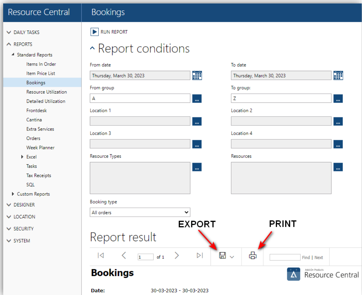
Figure 188. Bookings report
