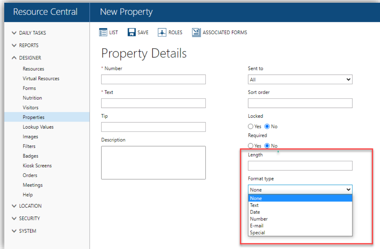
Figure 422. Property details
