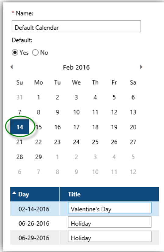
Figure 368. Choose Holiday
