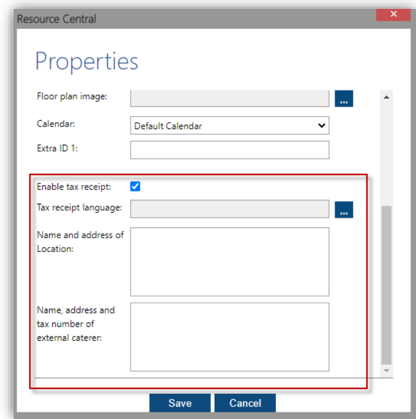
Figure 426. Location properties
