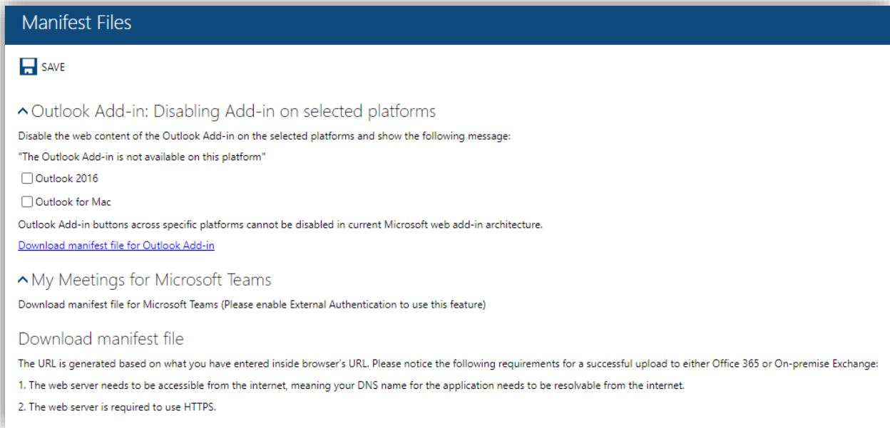
Figure 357. Manifest files
