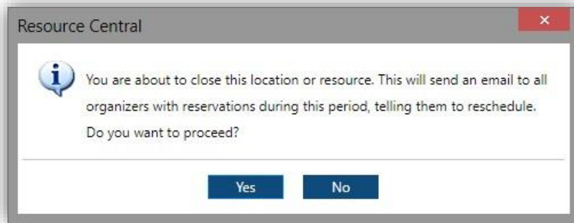
Figure 329. Closure prompt
