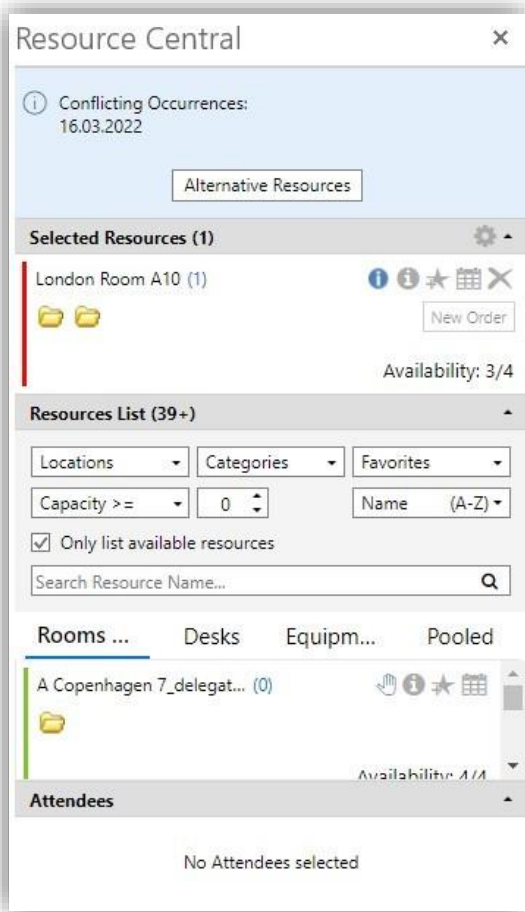
Figure 120. Alternative Resource
