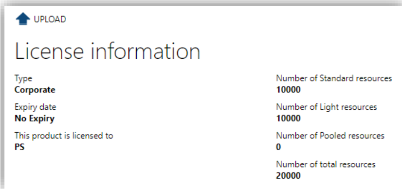
Figure 377. License Details
