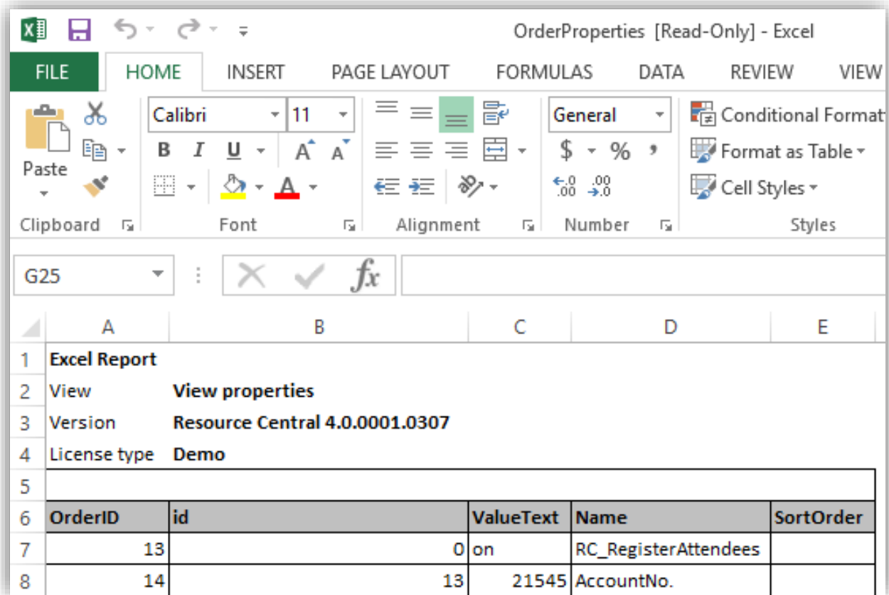
Figure 225. OrderProperties Excel
