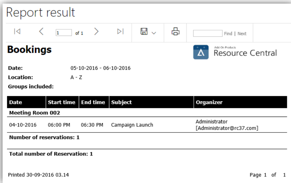
Figure 197. Bookings - report
