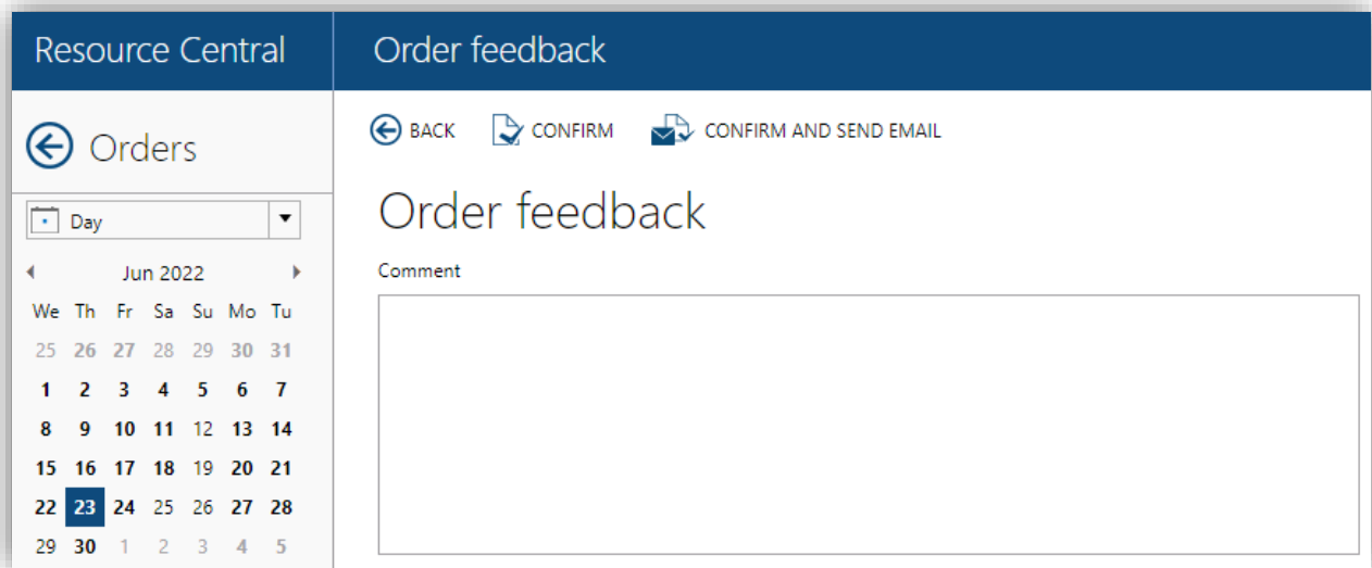
Figure 131. Order feedback
