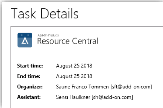
Figure 13. Task details
