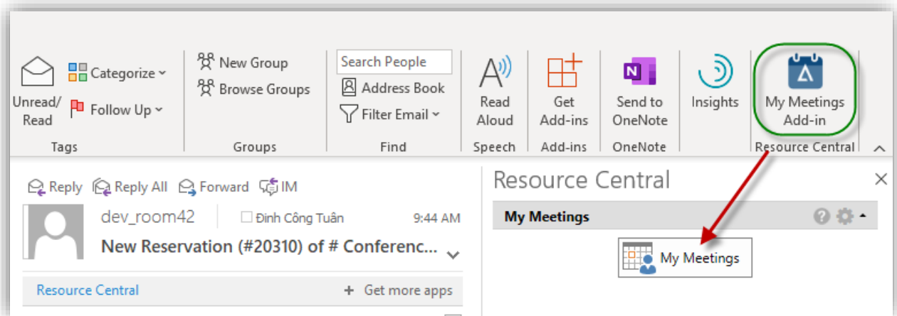
Figure 124. My Meetings
