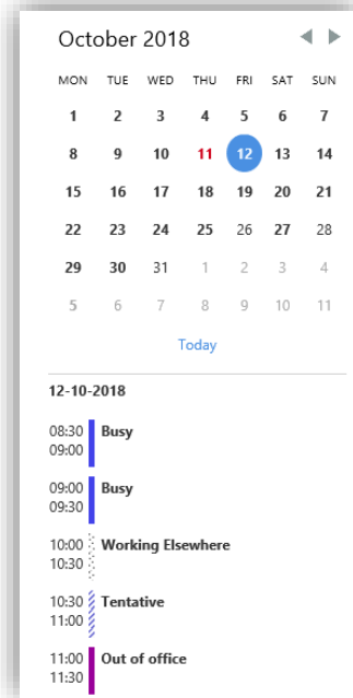
Figure 112. Attendee's calendar
