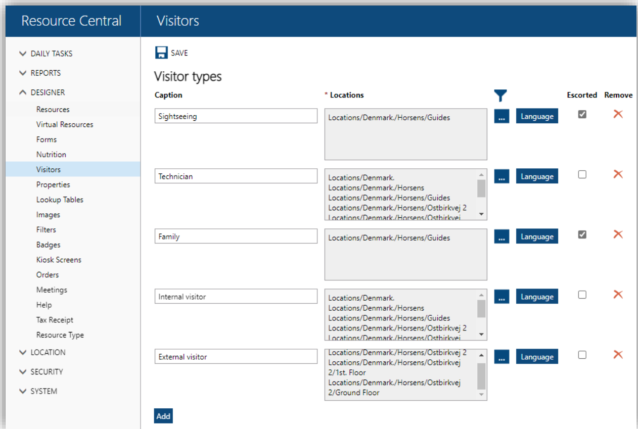
Figure 275. Visitor types
