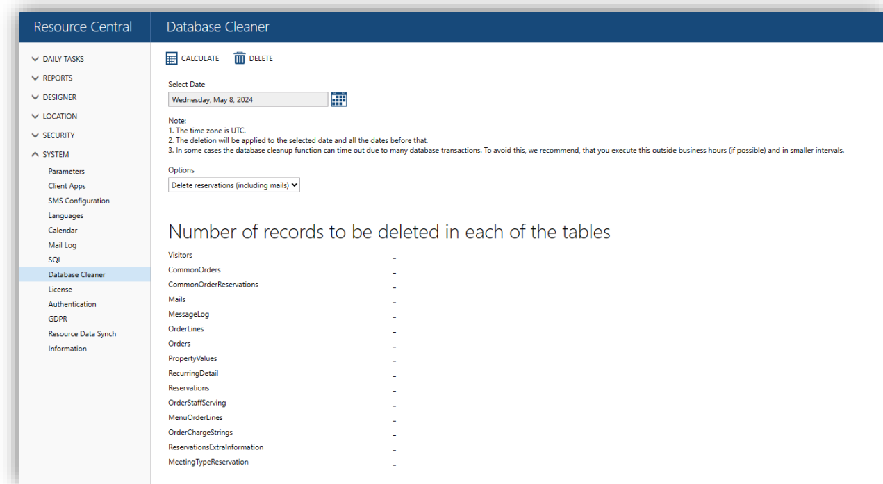
Figure 375. Database Cleaner
